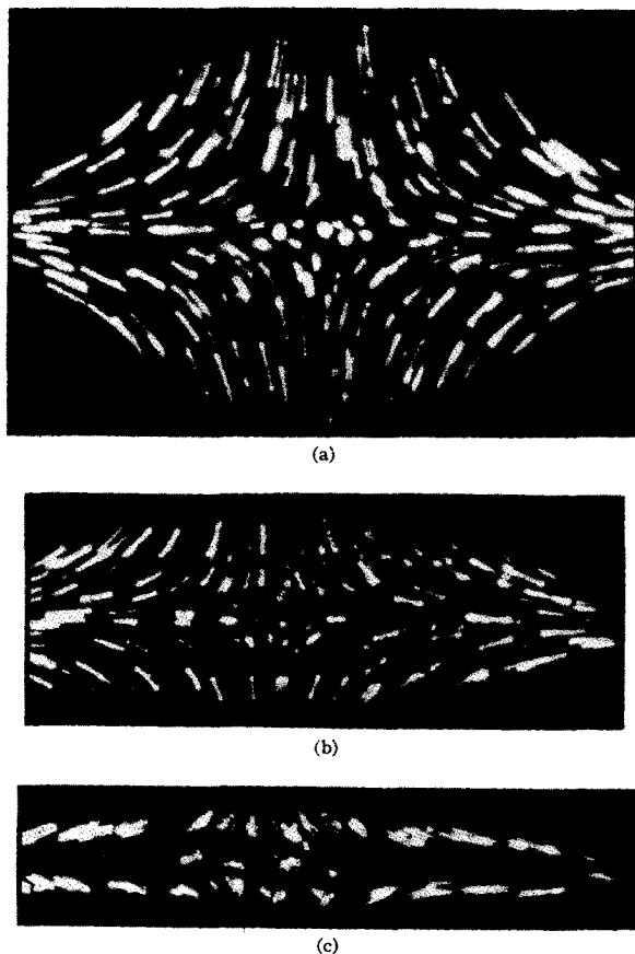
FIG. 10. Many body suspension viewed in the r - z plane. Experimental values: V_{ac}=500 v rms, \Omega=210 cy/sec. (a) Top picture: 2V_{dc}=-30 v, \omega_z=21.7 cy/sec; (b) Middle picture: 2V_{dc}=0 , \omega_z=26.0 cy/sec; (c) Bottom picture: 2V_{dc}=+24.7 v, \omega_z=29.4 cy/sec. The average charge to mass ratio of a single particle was e/m=0.00765 coulombs/kg.
