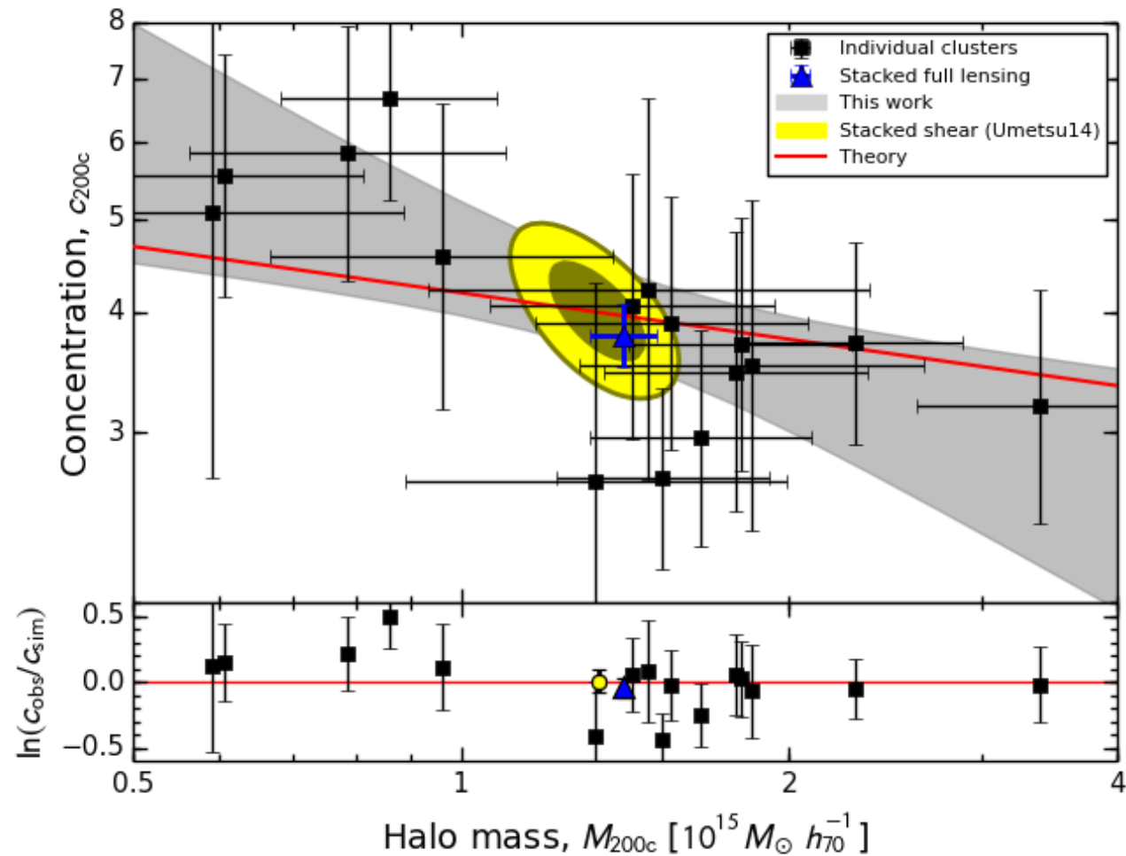
Halo concentration vs. mass relation
