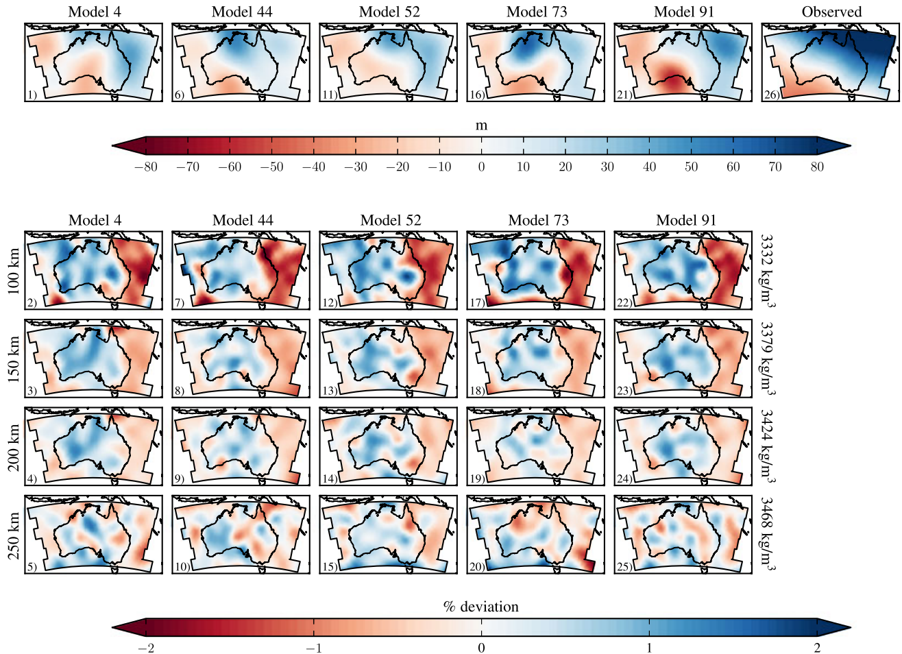
Figure 14. A selection of “best-fitting” (plots labeled “Model 4, 44, 52, 73, and 91”) and corresponding models of density anomalies in the upper mantle at depths of 100, 150, 200, and 250 km depth. For comparison, observed geoid anomaly is also shown (labeled “Observed”). Data fit is measured in terms of variance reduction and correlation to observed geoid anomalies (see Table 2 and main text for details).
