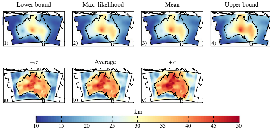
Figure 5. Maps of Moho depth (in kilometers) showing (plot 2) maximum likelihood model, (plot 3) mean model, and (plot 4) upper and (plot 1) lower bounds in the form of 95% highest probability density regions as measures of overall uncertainty on Moho depth obtained in the present study. Note that the maximum likelihood model is but one among many models that fit data. Plots in the bottom row display mean Moho depth (b) \pm one standard deviation ( \sigma ) (plots a and c) obtained by Bodin et al. [2012a] in their study of crustal structure based on a large diverse set of seismic data.
