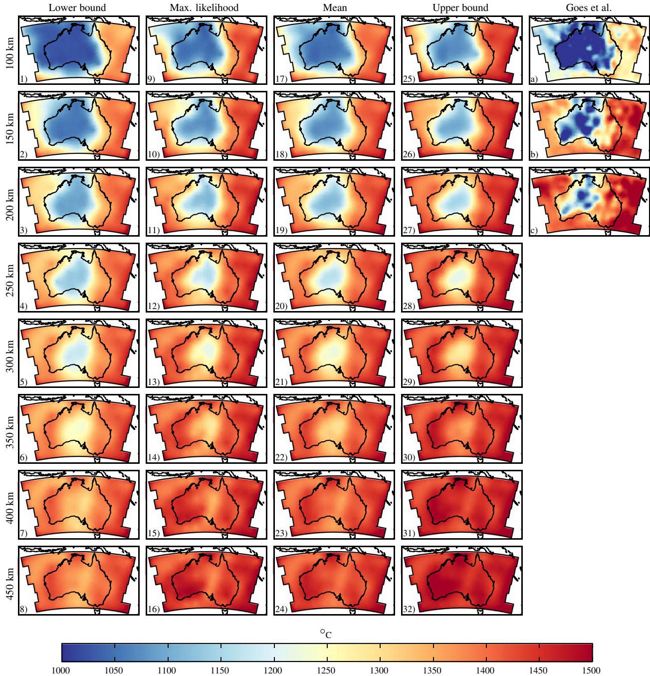
Figure 8. Maps of mantle temperature showing variations in temperature (in °C) at various depths underneath the Australian continent and surrounding oceans. (plots 9–16) Maximum likelihood model, (plots 17–24) mean model, (plots 1–8) lower bounds, and (plots 25–32) upper bounds, respectively, in the form of 95% highest probability density regions. Plots a–c show thermal maps derived by Goes et al. [2005]. See text for details.
