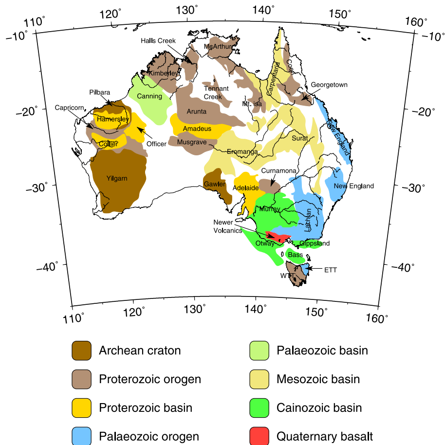
Figure 1. Simplified tectonic map of Australia.
