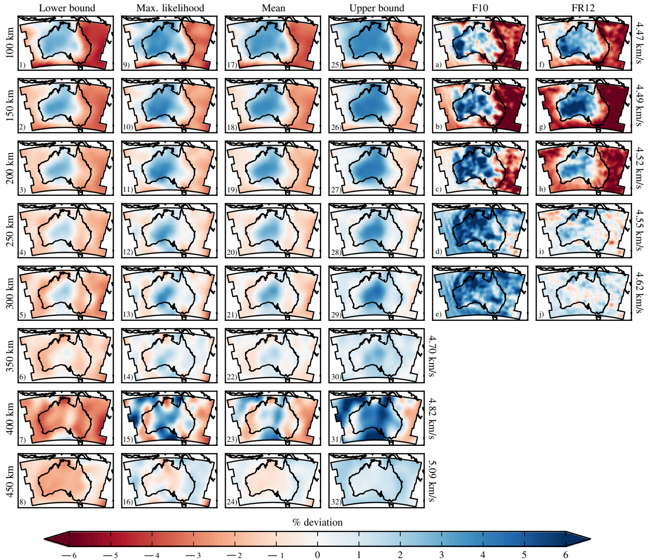
Figure 10. Maps of mantle isotropic shear-wave velocities showing variations in shear-wave speeds at various depths underneath the Australian continent and surrounding oceans. Shear-wave speeds are given in percent deviations from the mean shear-wave velocities computed here (see profile labeled AUS in Figure 11) and are indicated on the right side of the figure. Maximum likelihood model (maps 9–16), mean model (maps 17–24), lower bounds (maps 1–8), and upper bounds (maps 25–32), respectively, in the form of 95% highest probability density regions. Plots a–e depict the regional seismic full waveform tomography model of Fichtner et al. [2010], whereas plots f–j show the surface-wave tomography model of Fishwick and Rawlinson [2012].
