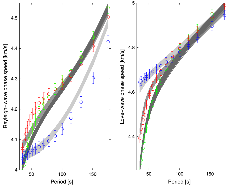
Figure 9. Comparison of calculated (gray lines) and observed Rayleigh- and Love-wave phase velocities (circles in red, blue, and green), including uncertainties (error bars in red, blue, and green) at an oceanic location (light gray/blue) and two continental locations (gray/red and dark gray/green) for the case of inversion with fixed mantle composition. Only fundamental-mode (left) Rayleigh- and (right) Love-wave branches are shown as these are consistently “misfit.” For details, see main text.
