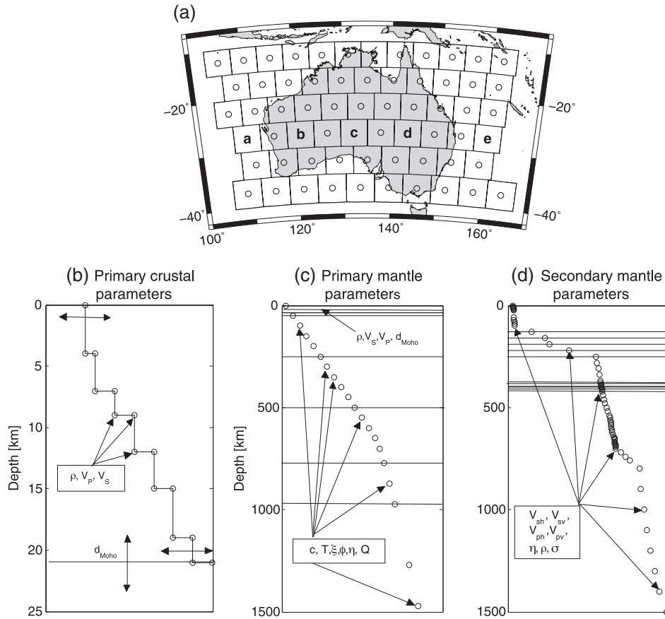
Figure 2. (a) Lateral and (b–d) radial model parameterization. (Figure 2a) Dots at the center of each pixel denote the locations at which properties are defined laterally with a grid spacing of 5^\circ \times 5^\circ . Letters a–e refer to locations for which radial shear-wave velocity profiles are displayed in Figure 11. Radially (Figures 2b–2d), the model is parameterized in terms of layers. The primary (fundamental) parameters are as follows: (Figure 2b) crust is delineated by density ( \rho ), P and S wave velocity ( V_p , V_s ), and depth to crust-mantle interface ( d_{\text{Moho}} ) while mantle layers (Figure 2c) are described by the main parameters: composition ( c ), temperature ( T ), anisotropy ( \xi , \phi , \eta ), and attenuation ( Q ). (Figure 2d) Secondary parameters (physical properties: V_{SH} , V_{SV} , V_{PH} , V_{PV} , \eta , and \rho ) are computed on the basis of the primary parameters on a grid, which is finely spaced around locations of major mantle mineral phase transitions. Circles in both plots denote location of a set of prefixed depth nodes, except in the crust where depth to crust-mantle interface is variable.
