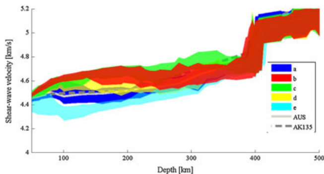
Figure 11. Shear-wave velocity profiles beneath different tectonic settings in the upper mantle and transition zone: Oceanic (pixels a and e) and continental (pixels b–d, with decreasing age progression from pixels b to d). Envelopes encompass all sampled models. Refer to Figure 2 for geographic location of pixels a–e. For reference, two mean radial models are also shown: AK135 [Kennett et al. , 1995] and the average profile (AUS) of the Australian continent computed as the mean of all sampled models across all pixels.
