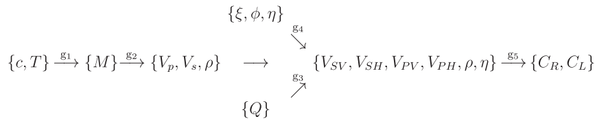
Figure 3. A schematic illustration of the forward problem and the different model parameters ( c, T, \xi, \phi, \dots ), physical theories ( g_1, g_2, \dots ), and data ( C_R, C_L ) used to describe it. Symbols are described in section 3.2.
