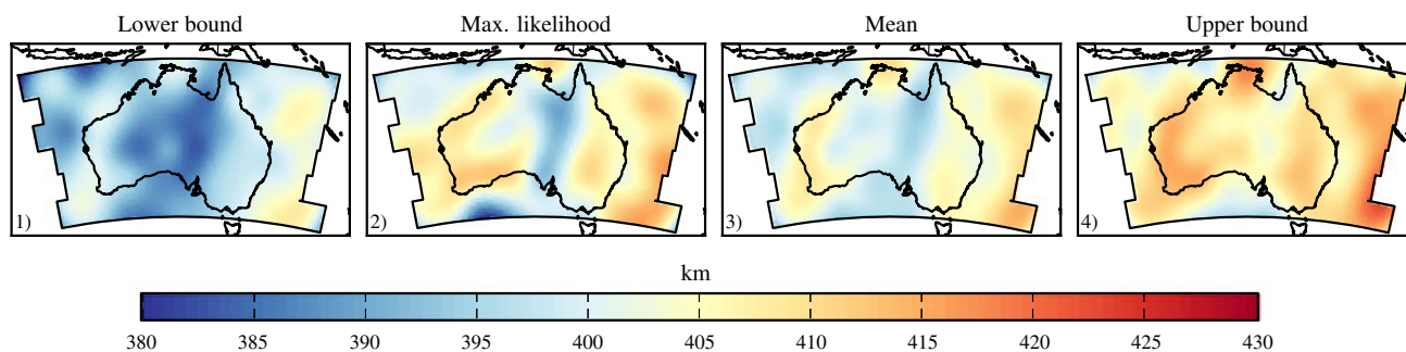
Figure 12. Depth to “410” km seismic discontinuity marking the transition between upper mantle and transition zone as defined by the mineral phase transition olivine→wadsleyite. Maximum likelihood model (plot 2), mean model (plot 3), and lower and upper bounds (plots 1 and 4) in the form of 95% highest probability density regions.
