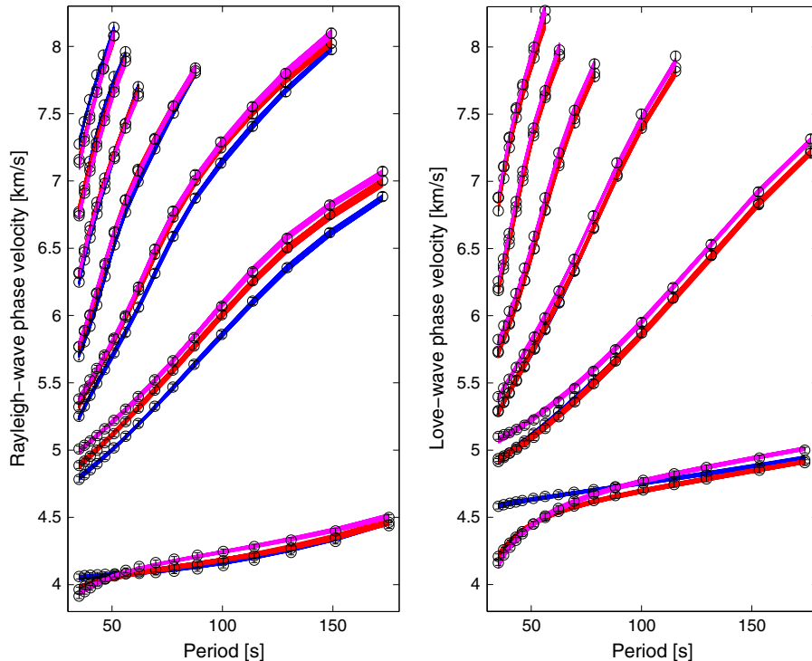
Figure 4. Comparison of calculated (red, blue, and magenta lines) and observed Rayleigh- and Love-wave phase velocities (circles), including uncertainties (error bars) at an oceanic (blue lines) and two continental (red and magenta lines) locations. Colored lines show calculated dispersion curves for all sampled models. Geographic location of sites is shown in Figure 2 as pixels a (blue), c (magenta), and d (red), respectively.
