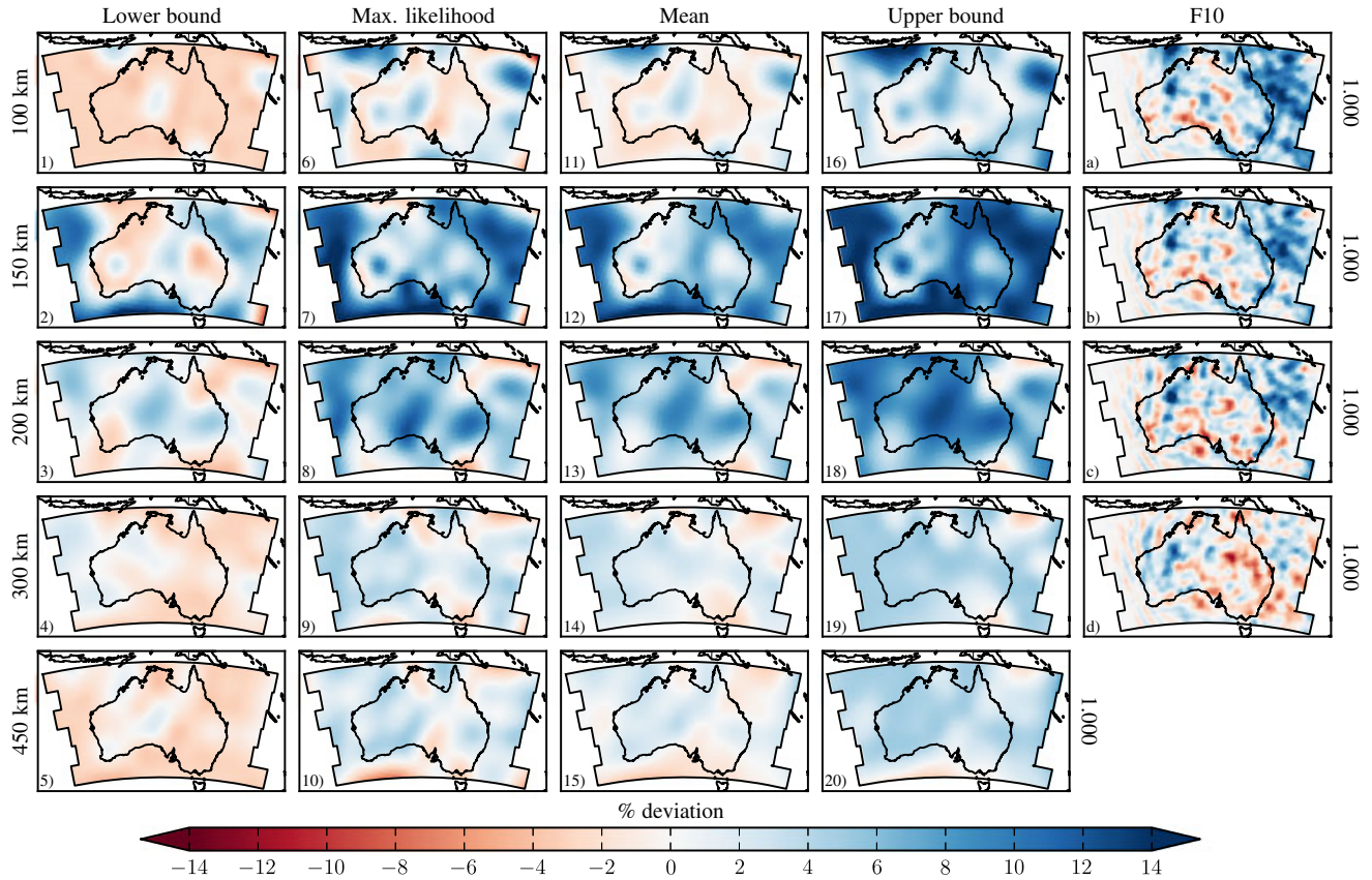
Figure 13. Maps of mantle shear-wave anisotropy variations ( \xi ) at various depths beneath the Australian continent and surrounding oceans. Shear-wave anisotropy is given in percent deviations from the mean (here \xi=1 ). Maximum likelihood model (plots 6-10) mean model (plots 11-15) lower bounds (plots 1-5), and upper bounds (plots 16-20), respectively, in the form of 95% highest probability density regions. Plots a–d depict shear-wave anisotropy variations in the full waveform tomography model of Fichtner et al. [2010].
