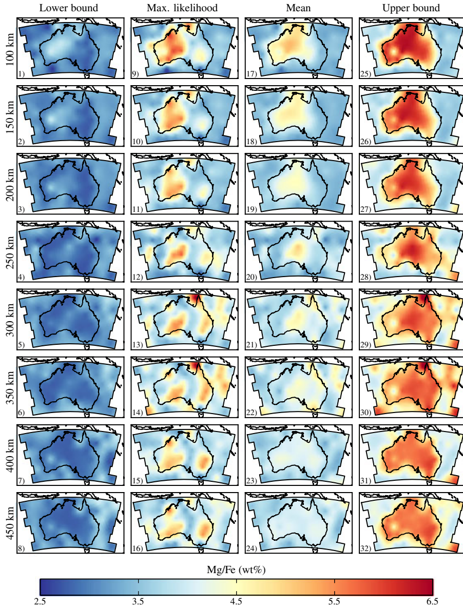
Figure 6. Maps of mantle composition showing variations in elemental Mg/Fe (wt %) at various depths underneath the Australian continent and surrounding oceans. (plots 9–16) Maximum likelihood model, (plots 17–24) mean model, (plots 1–8) lower bounds, and (plots 25–32) upper bounds, respectively, in the form of 95% highest probability density regions.
