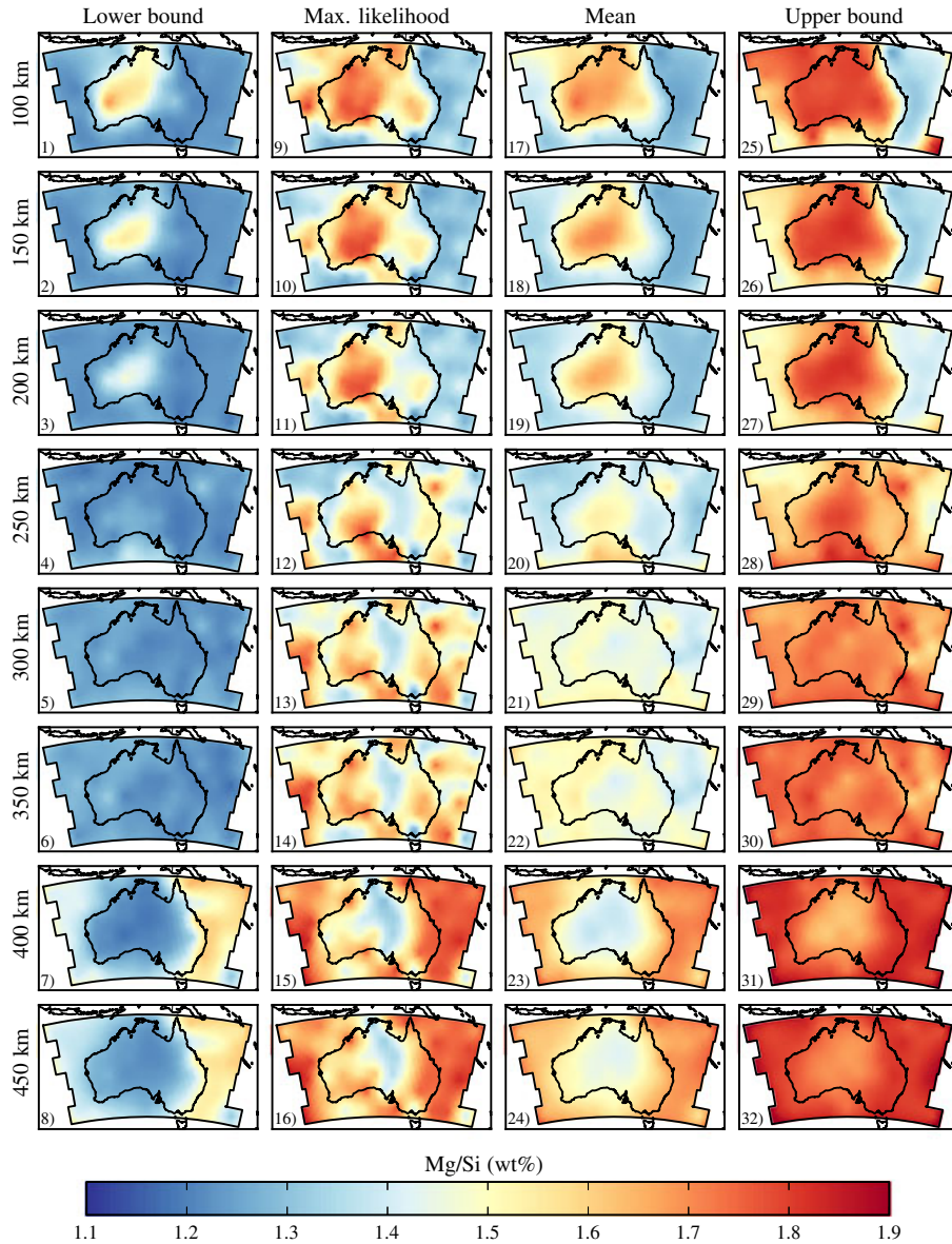
Figure 7. Maps of mantle composition showing variations in elemental Mg/Si (wt %) at various depths underneath the Australian continent and surrounding oceans. (plots 9–16) Maximum likelihood model, (plots 17–24) mean model, (plots 1–8) lower bounds, and (plots 25–32) upper bounds, respectively, in the form of 95% highest probability density regions.
