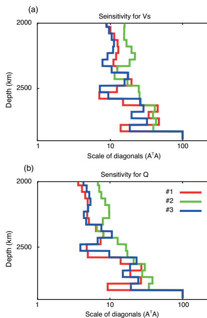
Figure 10. Sensitivity kernel for (a) V_S and (b) Q . Vertical axis shows depth. Horizontal axis indicates logarithm values of diagonal of A^T A corresponding to a partial derivative for a given depth. All values are normalized by the value at the largest depth. Each colour represents each data set, red: #1, green: #2 and blue #3.
