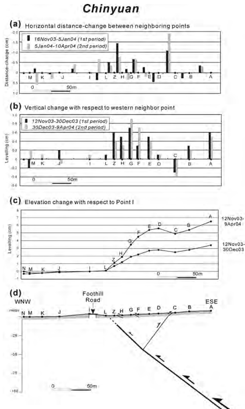
Figure 11. Results of distance-angle and leveling measurements across the surface fault zone of the Chihshang fault and geological interpretation at Chinyuan site. (a) Horizontal distance change between neighboring points. (b) Vertical change between benchmarks. (c) Elevation changes or vertical movements of benchmarks with respect to the point I. (d) Cross section showing surface ruptures, geometry of the fault, and slip model at the surface level. For further explanation, see Figure 5.
