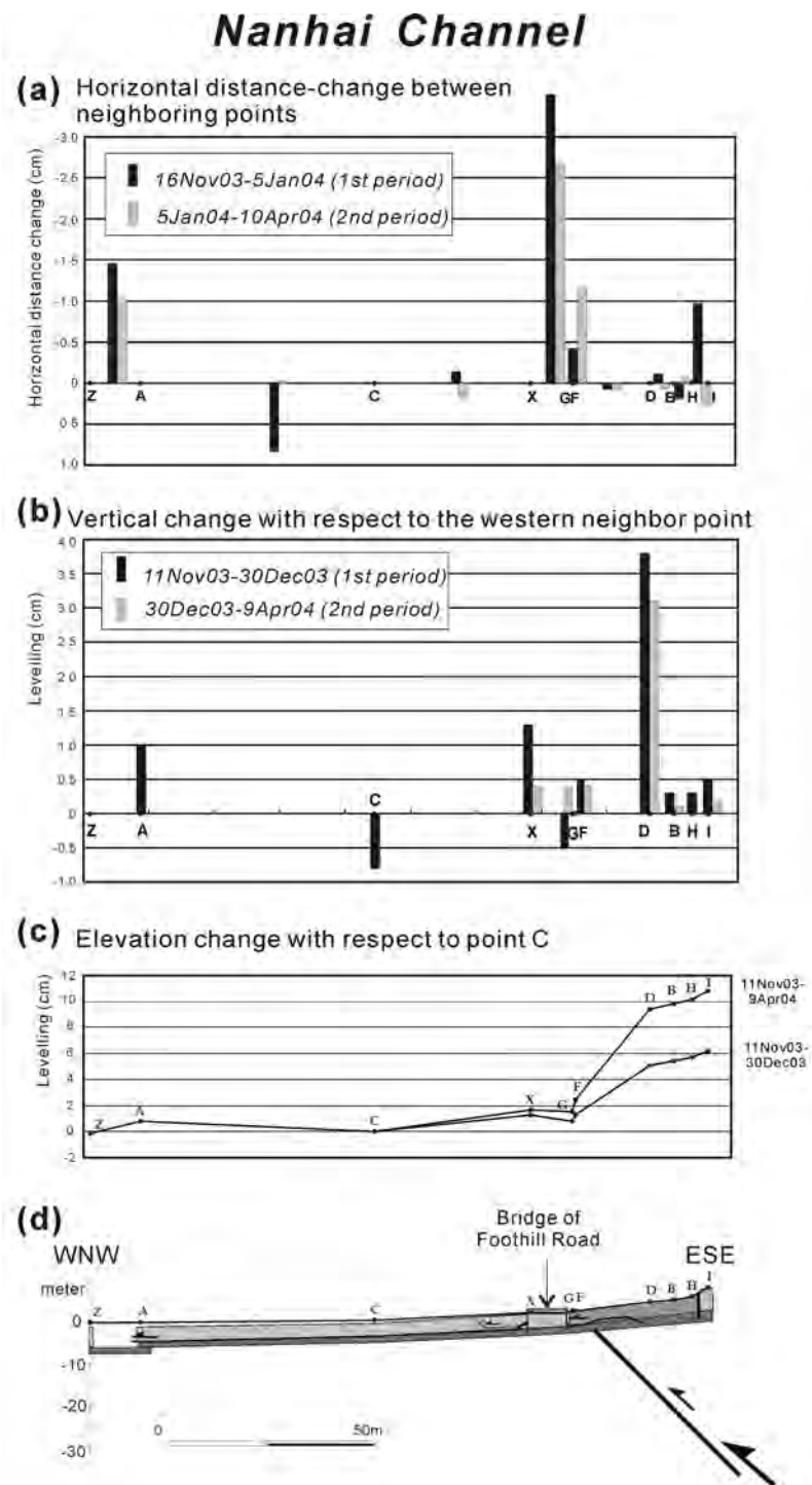
Figure 8. Results of distance-angle and leveling measurements across the surface fault zone of the Chihshang fault and geological interpretation at Nanhai channel site. (a) Horizontal distance change between neighboring points. (b) Vertical change between benchmarks. (c) Elevation changes or vertical movements of benchmarks with respect to the point C. (d) Cross section showing surface ruptures, geometry of the fault, and slip model at the surface level. For further explanation, see Figure 5.
