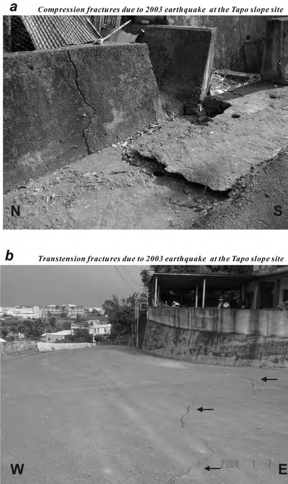
Figure 4. Photographs of the surface ruptures of concrete pavement along the roadside caused by the 2003 Chengkung earthquake at the Tapo slope site. (a) Pop-up-type or reverse fault-type fractures that indicate compression or shortening. (b) Open en échelon fissures (indicated by arrows) that show transension from near the top of the geomorphic scarp.
