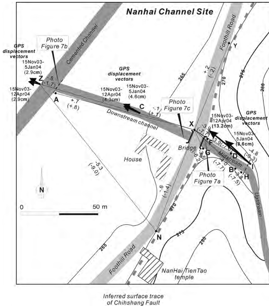
Figure 6. Results of horizontal distance changes and GPS horizontal displacements that occurred during the 2003 Chengkung earthquake at the Nanhai channel site. The contour lines show that the site is located across the scarp of the Chihshang fault and that the surface trace of the fault is approximately consistent with the foothill road. The values between the benchmarks indicate the measurement of horizontal distance changes. The GPS displacement vectors are with respect to a continuous GPS station SHAN in the Longitudinal Valley. For further explanation, see Figure 3.
