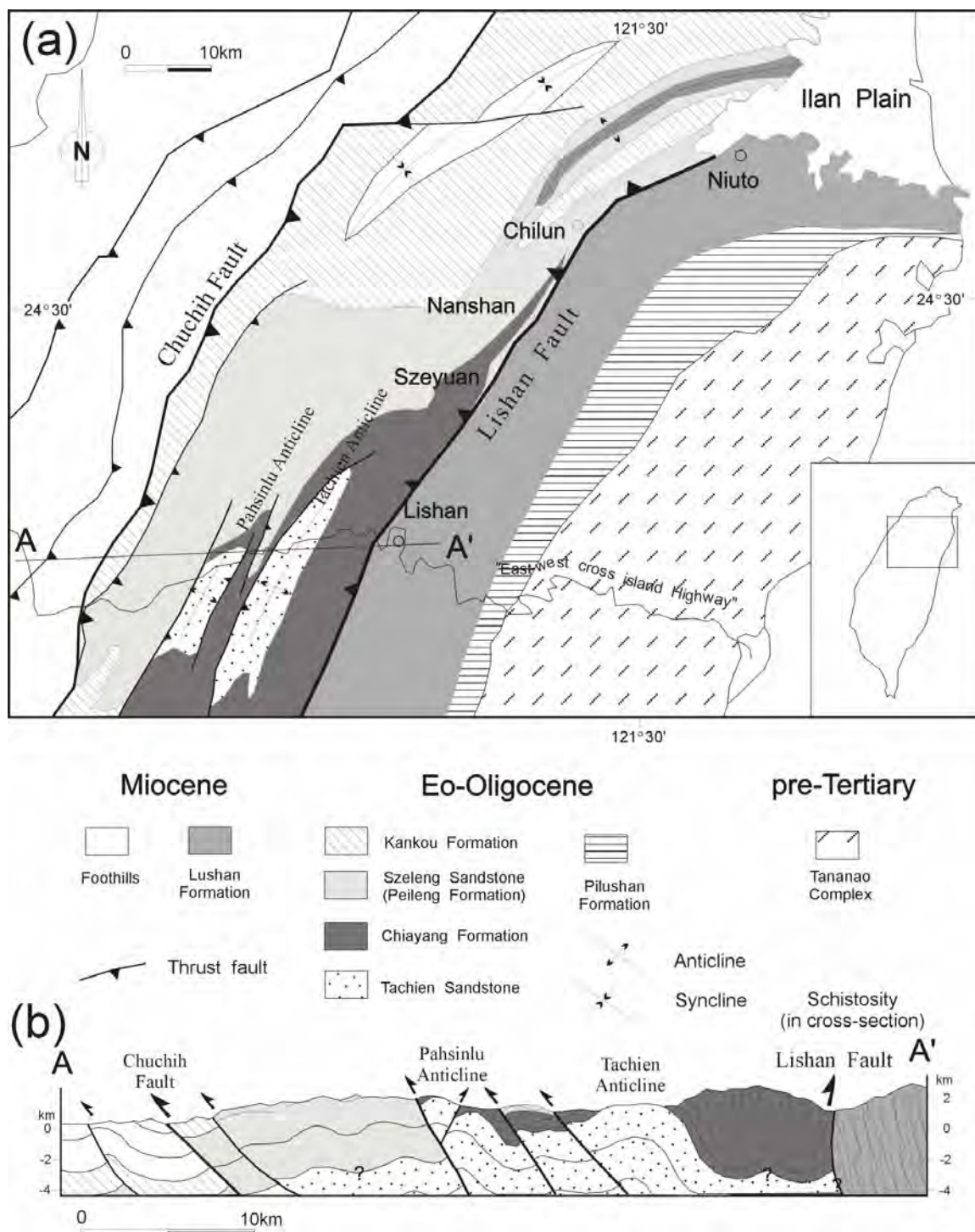
Fig. 2. (a) Geological map of the Lishan Fault region (after Ho, 1986b). (b) cross-section (AA', see location in a).
