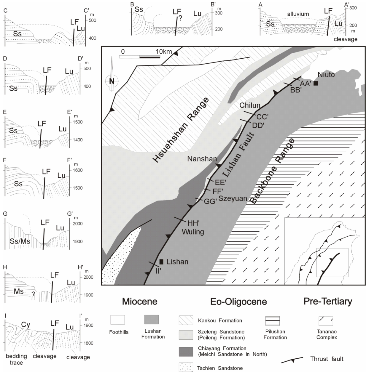
Fig. 3. Serial cross-sections across the Lishan Fault zone. In sections: Ss, Szeleng Sandstone; Ms, Meichi Sandstone; Cy, Chiayang Formation. Lu, Lushan Formation. Details in Table 1.
