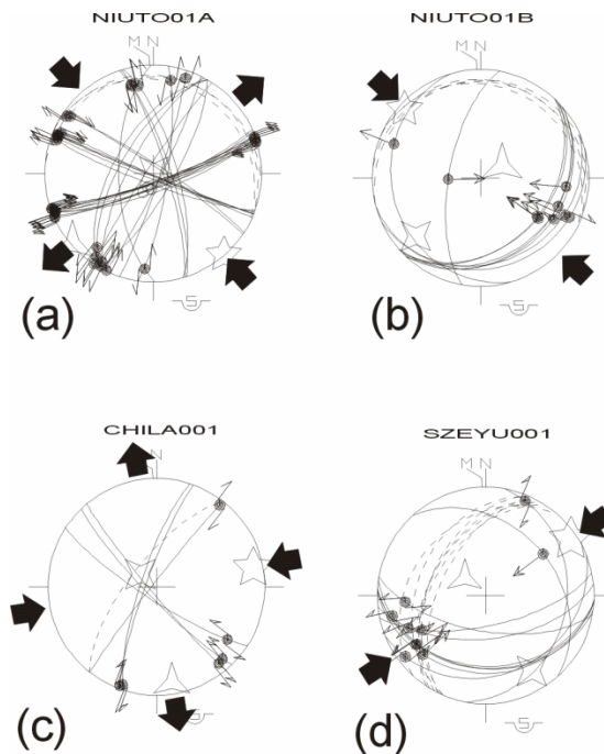
Fig. 5. Examples of stress tensor determination in the area of the Lishan Fault. Stereoplots: Schmidt's projection, lower hemisphere. Bedding planes shown as dashed-line great circles. Fault planes shown as thin great circles, with slickenside lineations as dots with arrows indicating the sense of motion (inward direction for reverse slip). Computed stress axes shown as stars with five branches ( \sigma_1 ), four branches ( \sigma_2 ), and three branches ( \sigma_3 ). Method of calculation of stress tensor: Angelier (1984). (a) Major NW-SE compression, strike-slip faulting (Niuto, location in Fig. 7). (b) Major NW-SE compression, reverse faulting (same site). (c) Minor NE-SW compression, strike-slip faulting (Chilun, location in Fig. 7). (d) Minor NE-SW compression, oblique reverse faulting (Szeyuan, location in Fig. 7 and backtilting in Fig. 6c). Numerical results given in Table 2.
