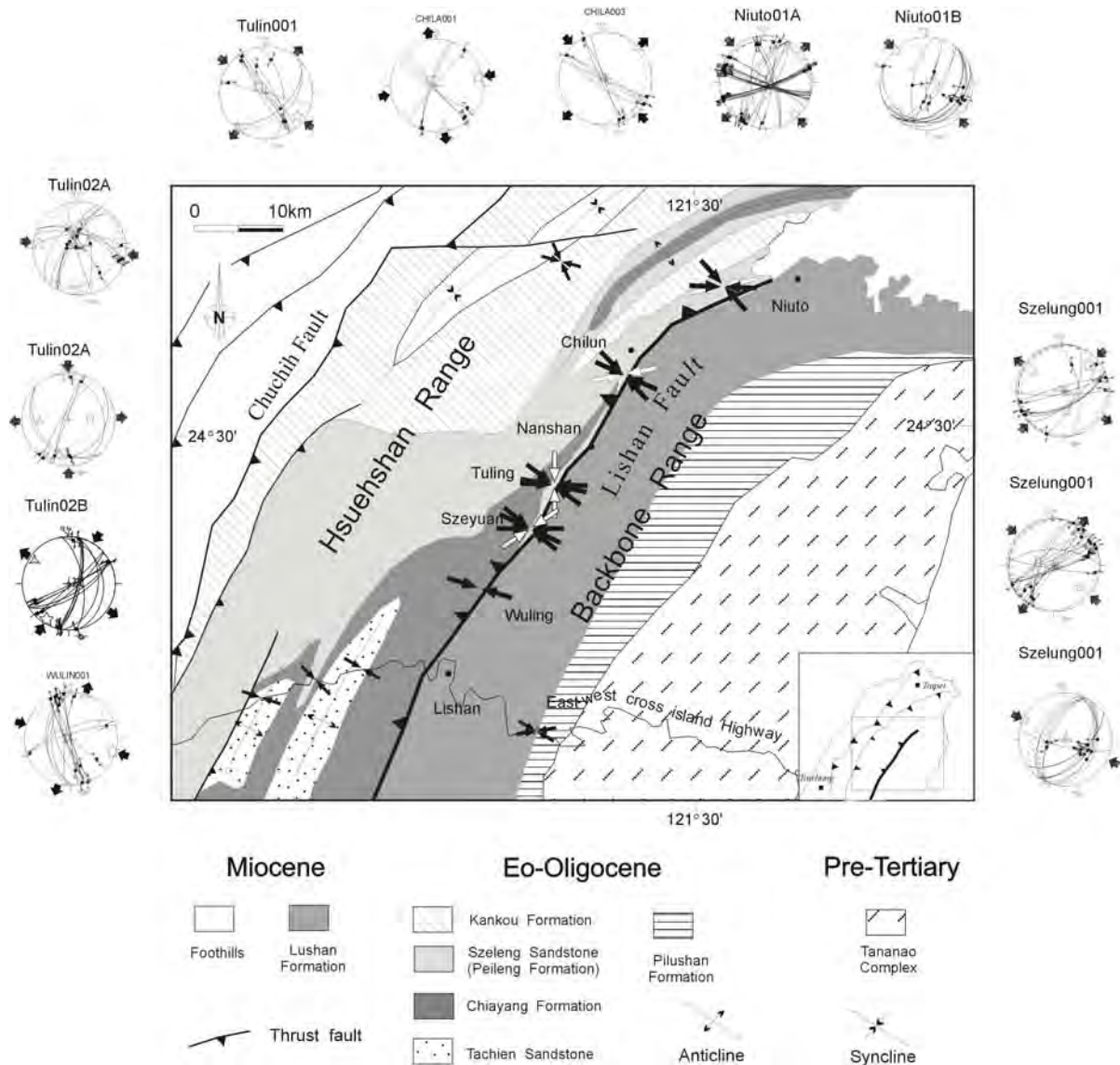
Fig. 7. Distribution of the direction of compression based on the results of paleostress analysis in the area of the Lishan Fault. Solid arrows, directions of compression ( \sigma_1 ) for the major event. Open arrows refer to the minor event of WNW-ESE compression and to the occurrence of N-S compression at Tuling. Numerical results in Table 2.
