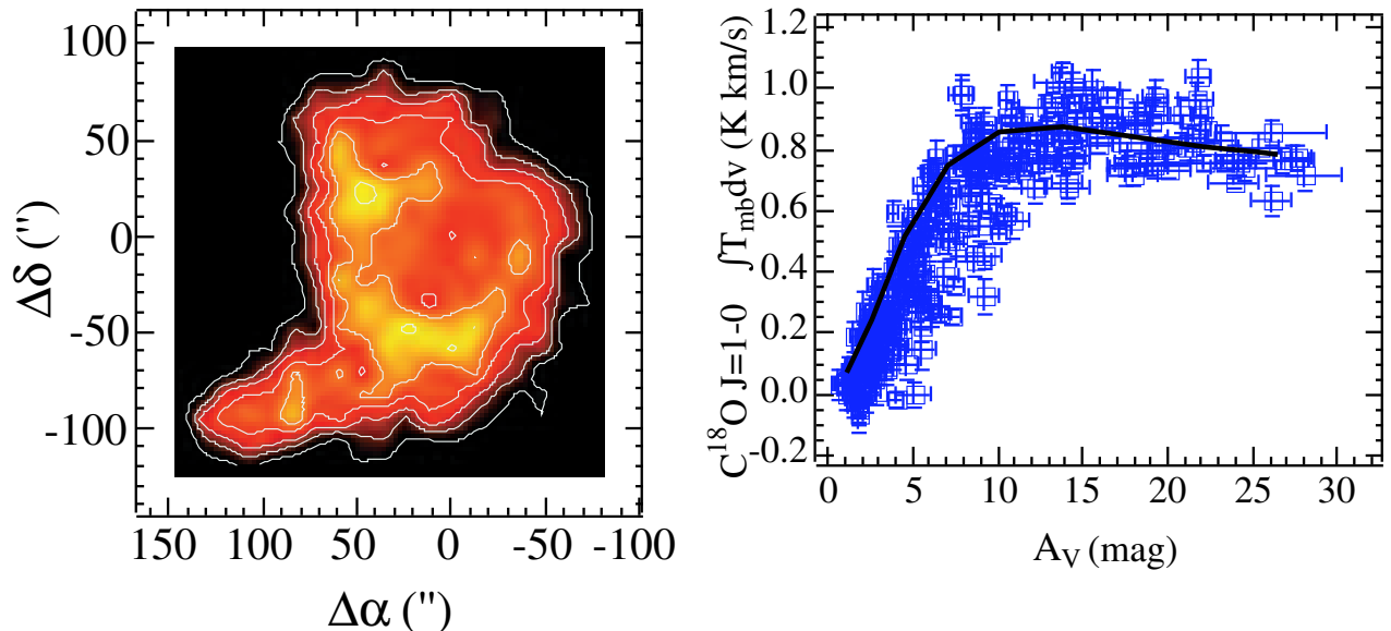
Fig. 6.— Map of C^{18}O (J=1-0) emission from the B68 cloud (left) together with a plot of the correlation between CO integrated intensity and extinction for the cloud (right). The break from a linear correlation at 10 magnitudes in the latter plot indicates a sharp decrease of CO abundance in the high extinction regions. This drop in abundance in the central regions is also manifest in the spatial map where a bright ring of emission surrounds a central depression. The solid line in the right hand plot represents the prediction of a chemical model in which the CO abundance is decreased by two orders of magnitude in the central regions of the cloud due to depletion onto grains (from Bergin et al., 2002 ).
