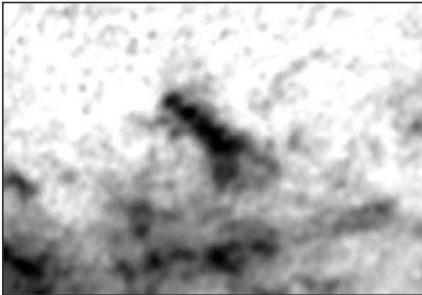
Dust extinction
